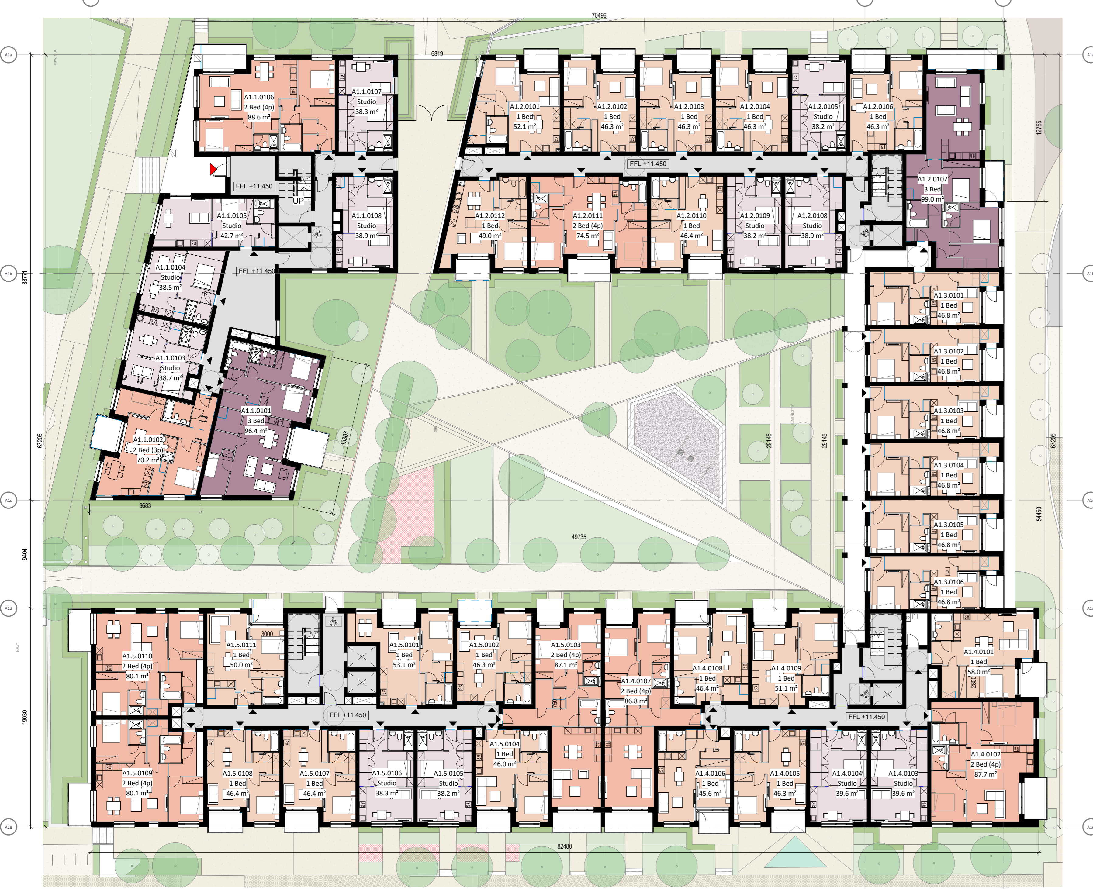
3 BLOCK A1 - LEVEL 01 1:200
